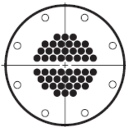
Full Face Tubesheet With Drilled Bolt Pattern
